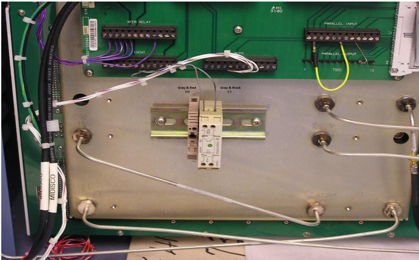
Wiring connection for new 046C05-0005 optic coupler
