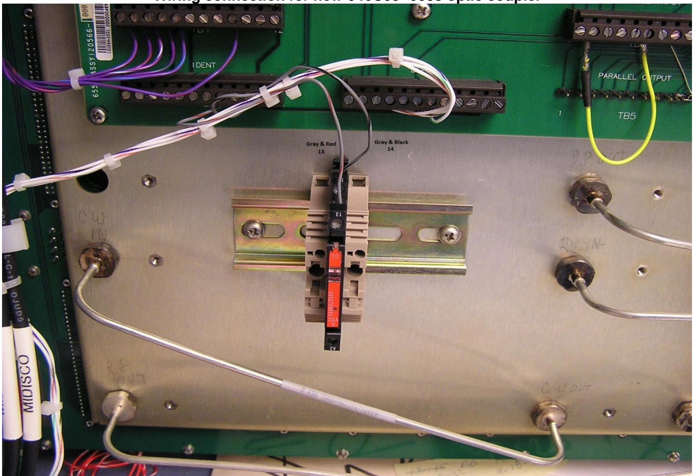
Wiring connection for new 046C05-0005 optic coupler
